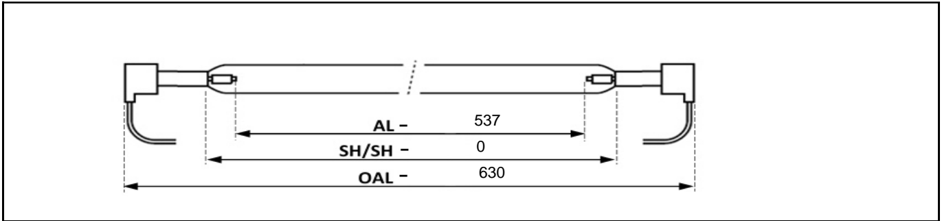
Socket Diagram:
